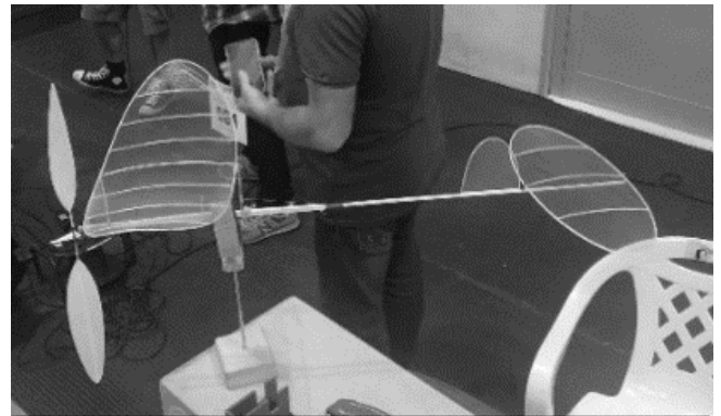
Jorge Garcia F1M-L with elliptical wing
