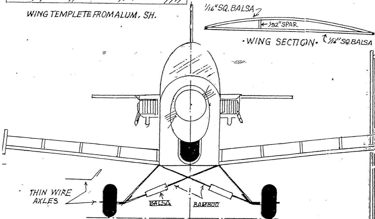
FRONT VIEW SKETCH
